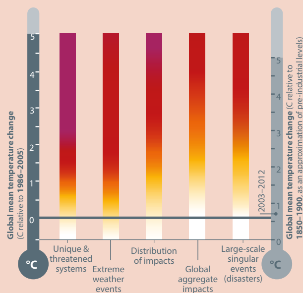
Level of additional risk due to climate change
