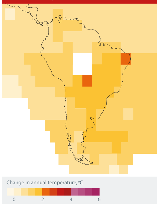
Figure 1: Change in annual average temperature in Latin America, 1901–2012 16
