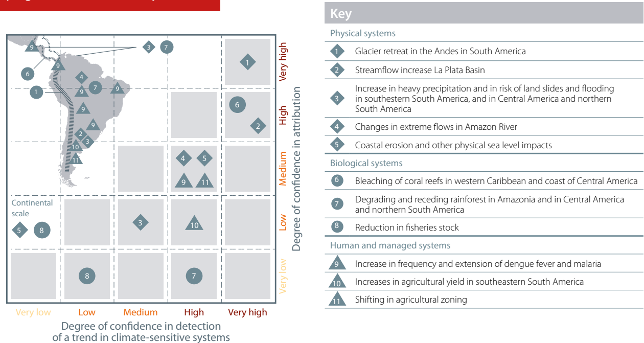
Figure 3: Role of climate change in shaping natural and human systems 26
