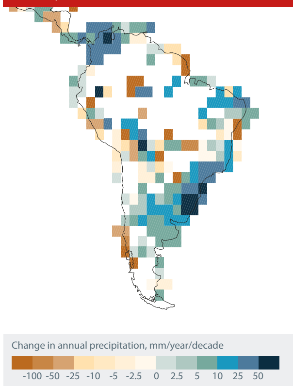
Figure 2: Change in annual average rainfall in Latin America, 1951–2010 17
