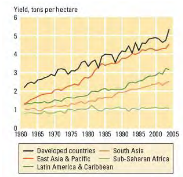
Figure 3.1: Evolution of cereal yields since 1960 across regions
